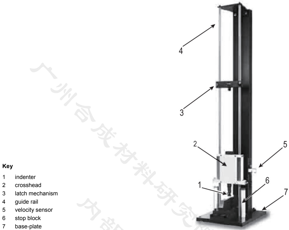
Figure 2 — Instrumented drop-weight impact device with double guide rails
