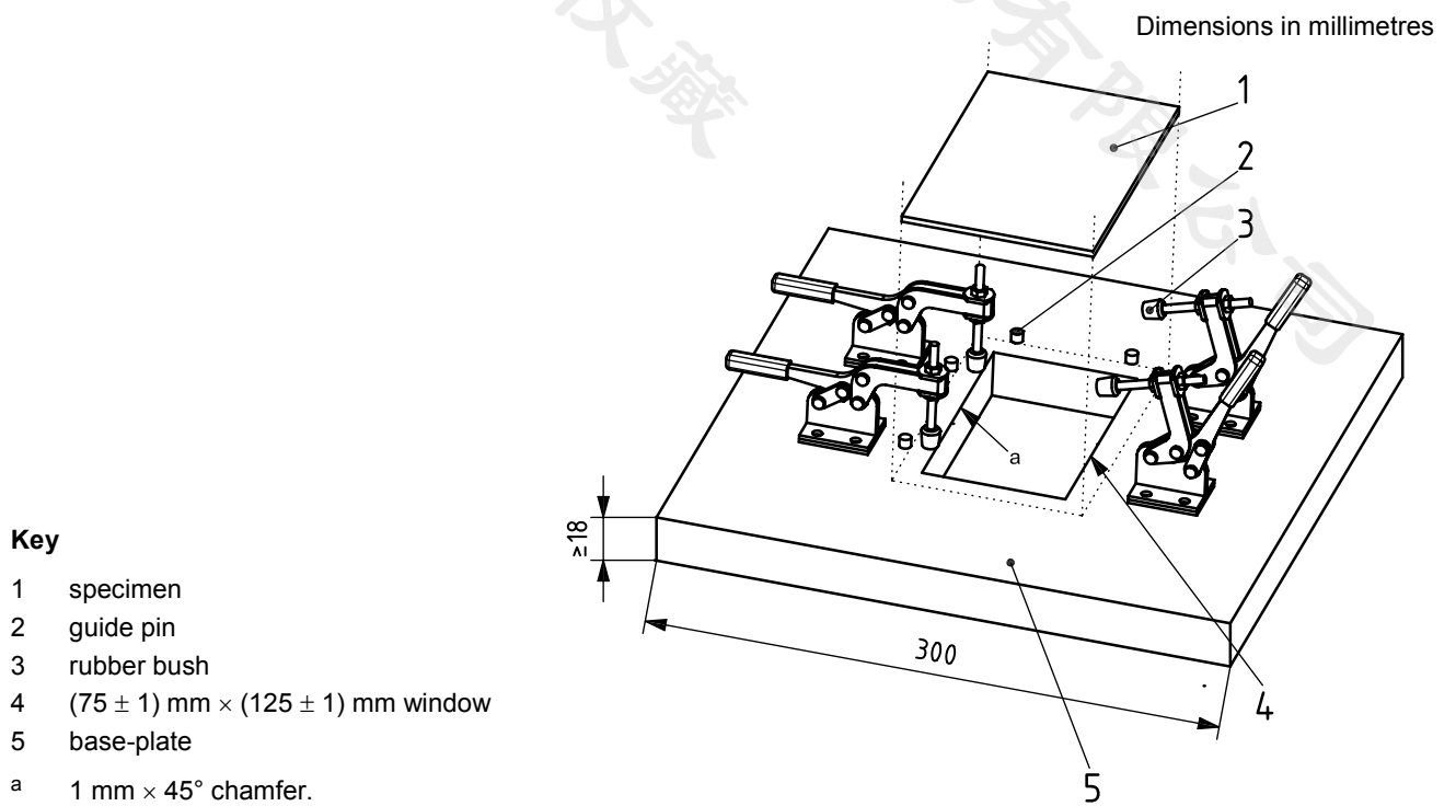
Figure 3 — Example of a specimen support fixture
