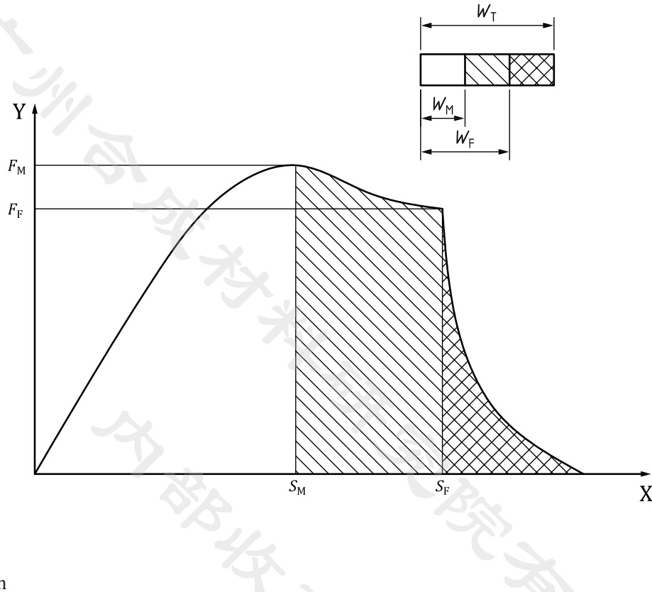
Figure 1 — Force-deformation diagram for very tough materials (schematic)
